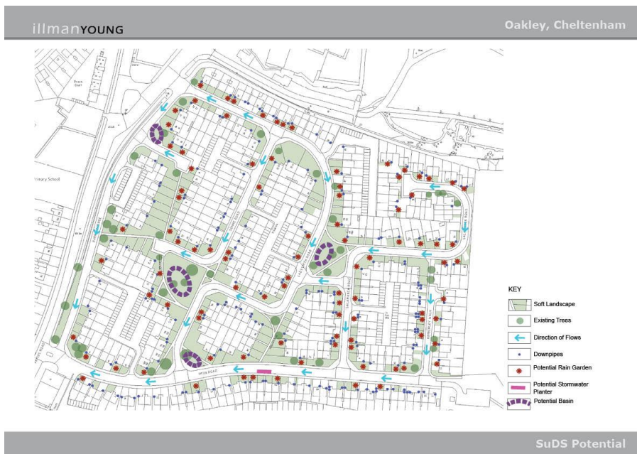
Fig 1: Potential Locations for SuDS features on Priors Farm Estate
