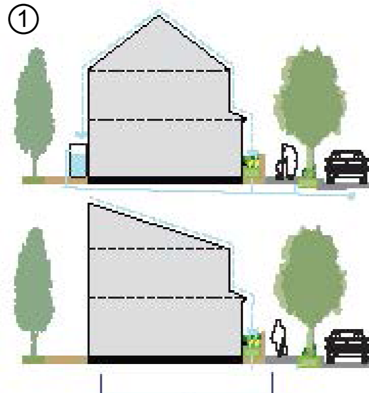
Roof drainage and SuDS options
